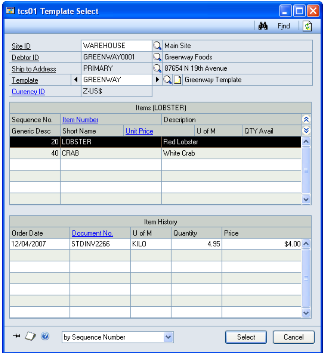
The Template Select window – Catchweights version
